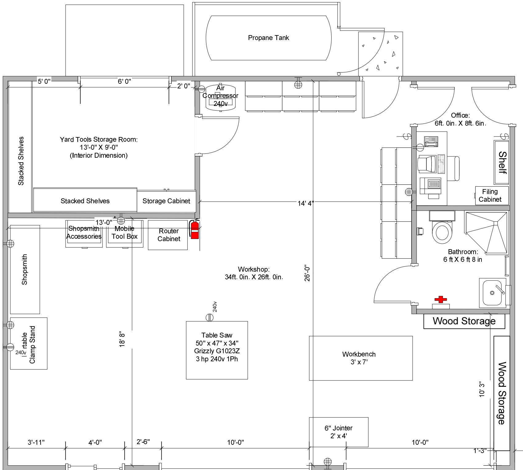
Conner Workshop scale: 1/4" = 1'
