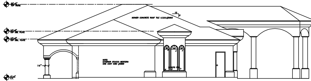
EAST ELEVATION SCALE 3/16"=1'-0"
